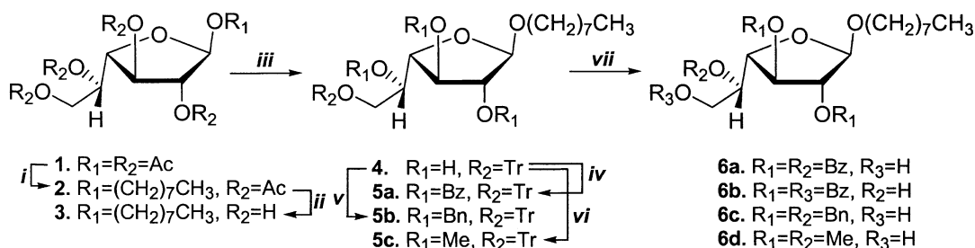
Scheme 1. Synthesis of various galactofuranosyl acceptors for \beta 1 \rightarrow 6 disaccharides. Reagents & Conditions: (i) SnCl 4 , CH 3 (CH 2 ) 7 OH, CH 3 CN, 0°C-rt, 30 min, 72%; (ii) NaOMe, MeOH, rt, 7 h, 95%; (iii) TrCl, Py, 50°C, 48 h, 72%; (iv) BzCl, Py, rt, overnight, 87%; (v) BnBr, NaH, DMF, 0°C-rt, 3 h, 99%; (vi) Mel, NaH, THF, rt, overnight, 90%; (vii) CH 3 COOH, H 2 O, 60°C, 30 min, 6a : 58%, 6b : 39%, 6c : 78%, 6d : 99%.
