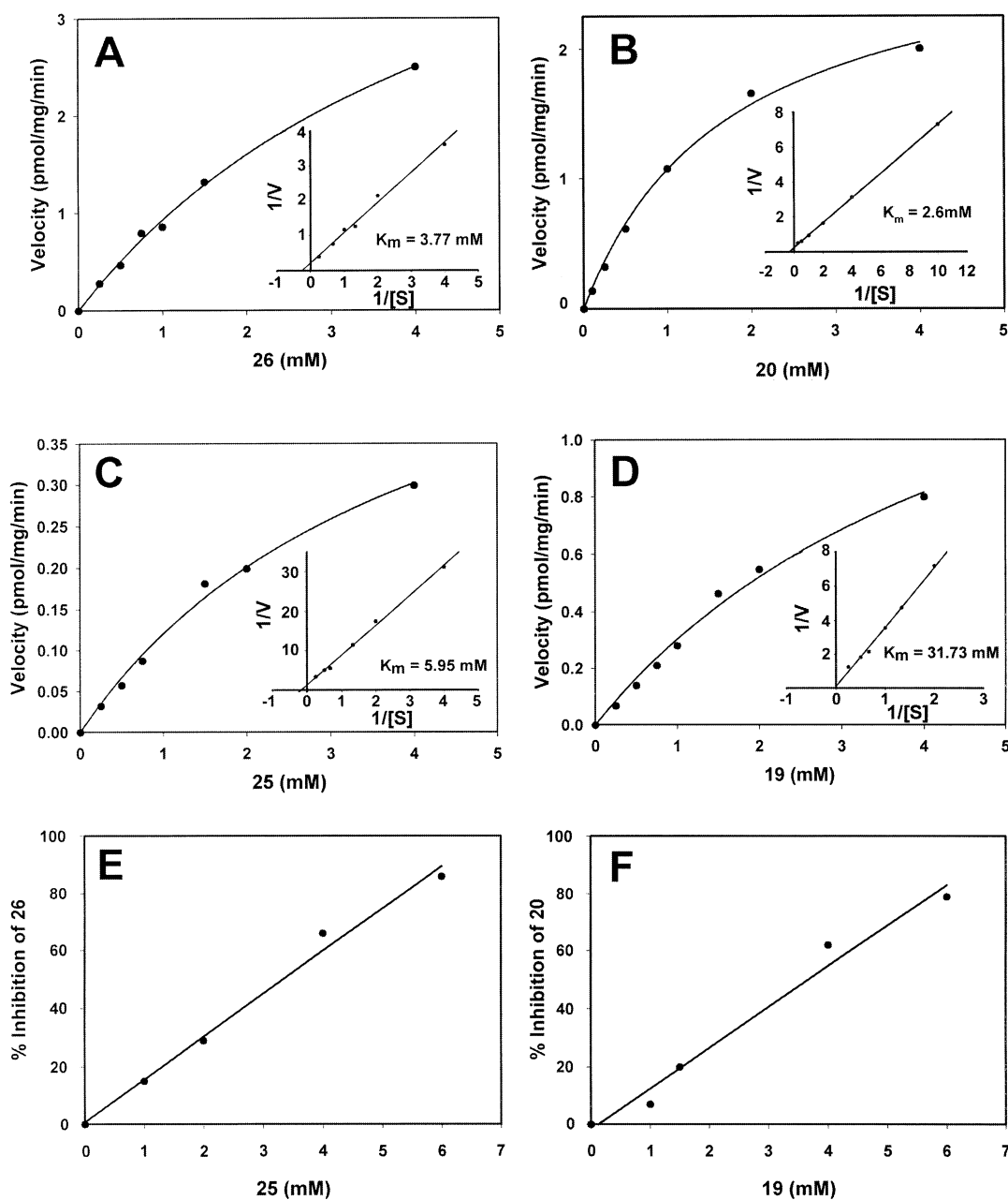
Figure 4. Kinetic analysis of acceptors 26 (panel A), 20 (panel B), 25 (panel C) and 19 (panel D). The insets illustrate the double reciprocal plots for each compound. The inhibitory properties of acceptors 25 (panel E) and 19 (panel F) are shown in a dose-response with compounds 26 and 20 at a fixed concentration of 0.5 mM, respectively.
