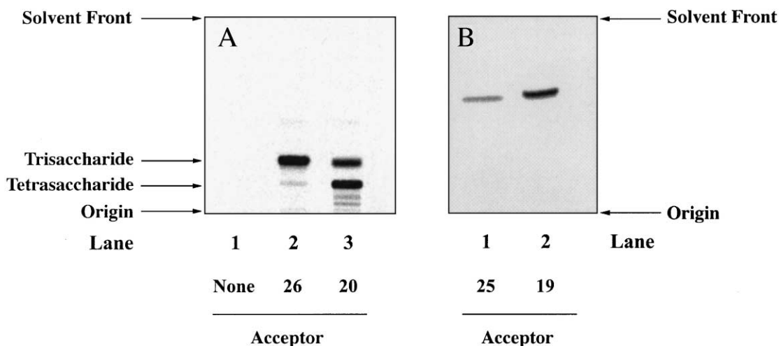
Figure 5. An autoradiogram of reaction products produced through the inclusion of 26 and 20 (panel A), and 25 and 19 (panel B), mycobacterial membranes and UDP-[ ^{14}\text{C} ]Gal. TLC/autoradiography was performed using chloroform/methanol/ammonium hydroxide/water (65:25:0.5:3.6) and products revealed through exposure to Kodak X-Omat film at -70^\circ\text{C} for 48 h.
